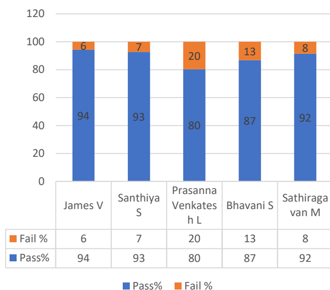
MA23434 OptimizationTechniquesforAI
