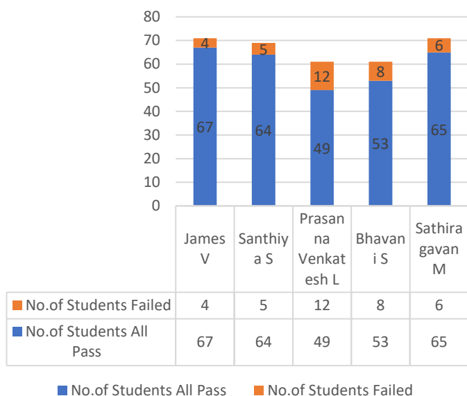
MA23434 OptimizationTechniquesforAI
